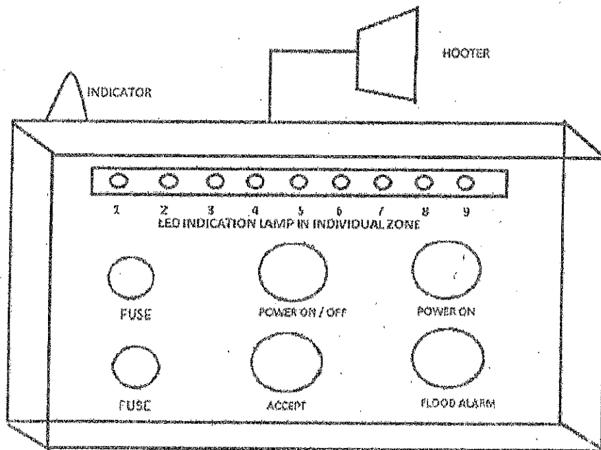
PROPOSED NEW CONTROL PANEL IN DINING HALL
