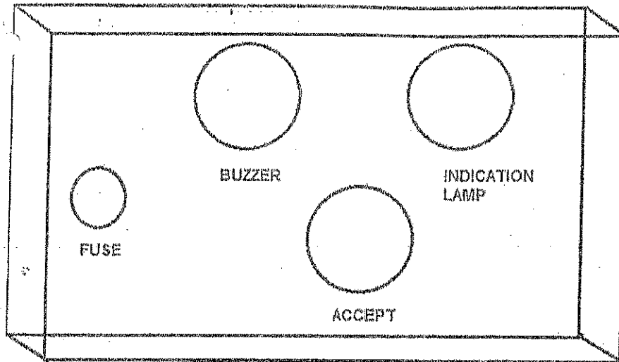
PROPOSED FLOOD SENSOR INDICATION PANEL IN BRIDGE
